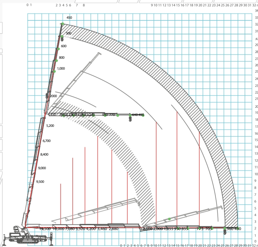
Load diagram with direct hook and jib
