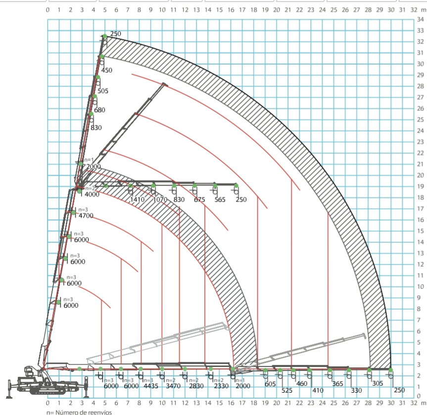
Load diagram with winch and jib
