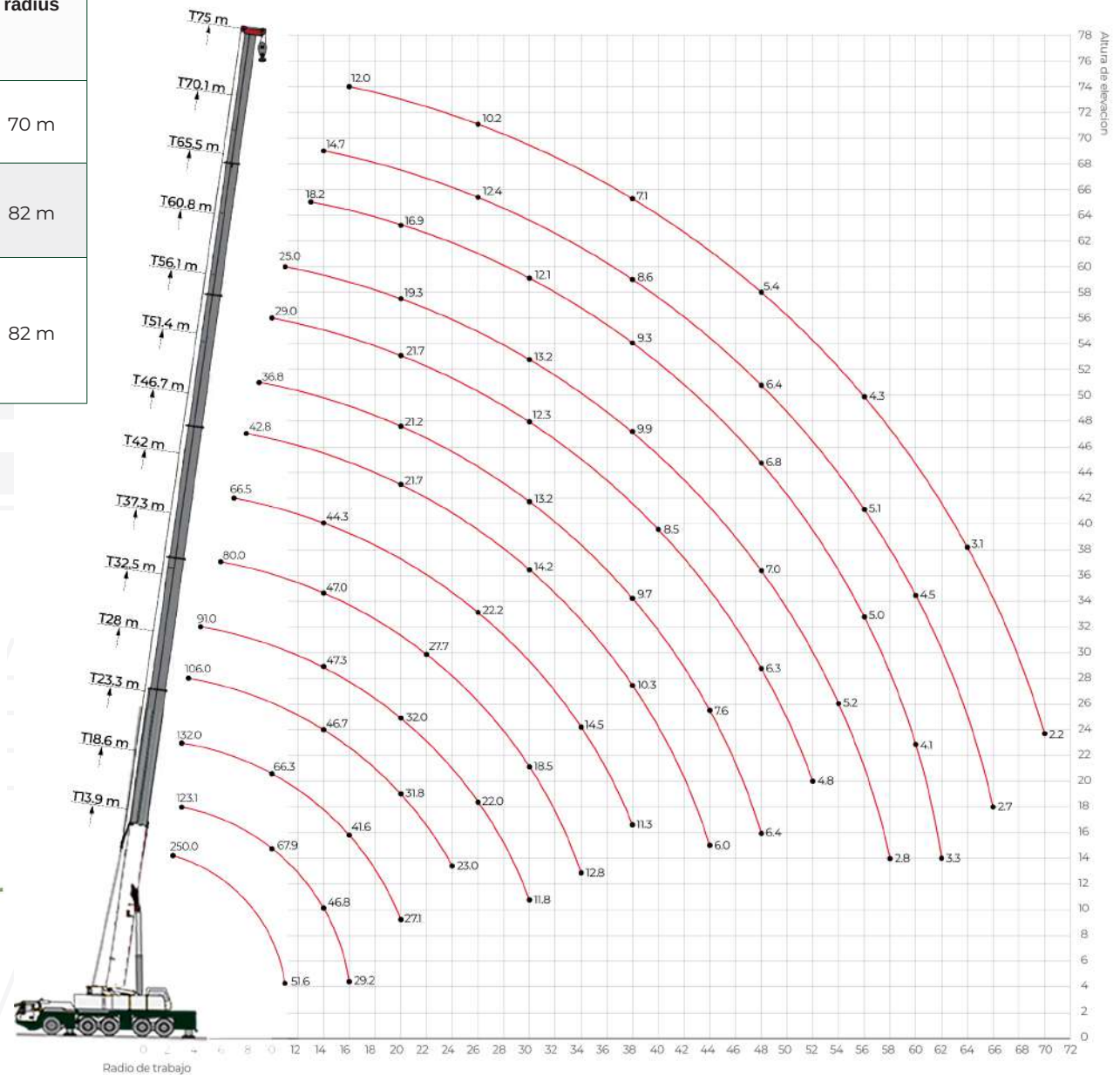
Load chart T
