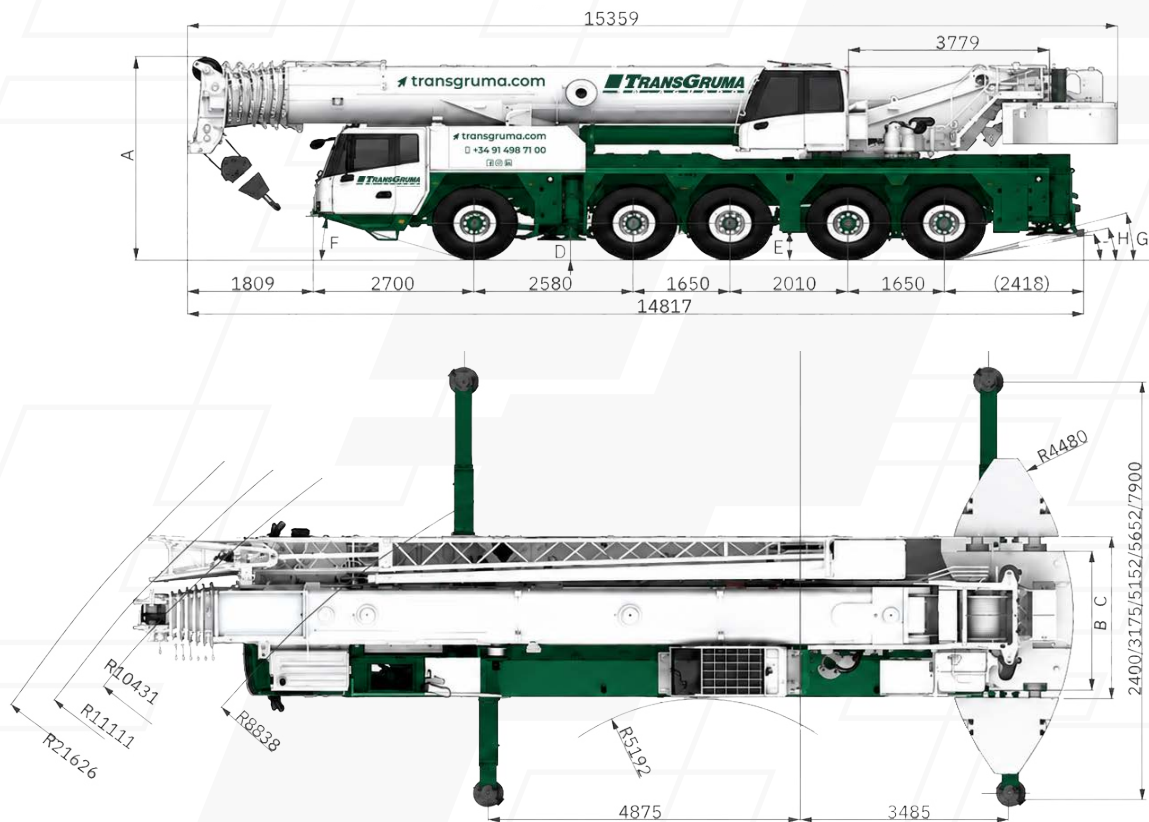
Telescopic crane dimensions
