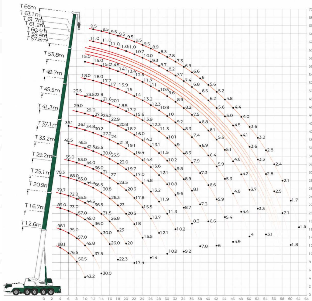
Load chart T
