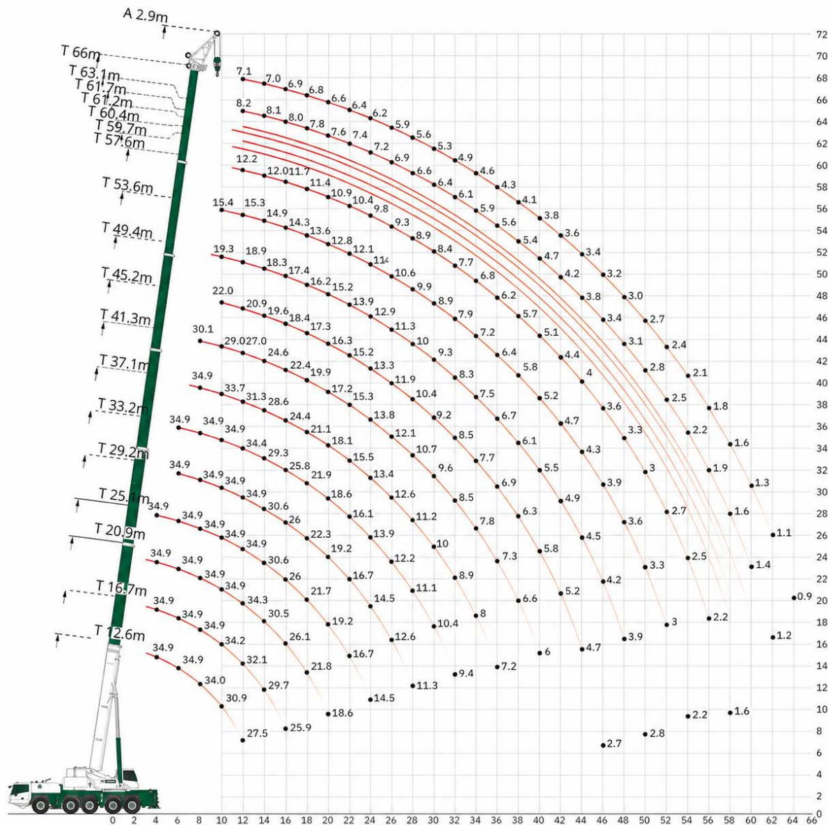
Load chart TA
